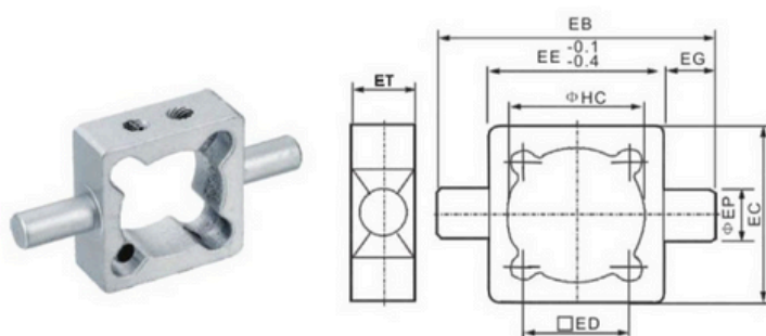
ISO-TC 型(Type)中摆(Central Trunnion)
